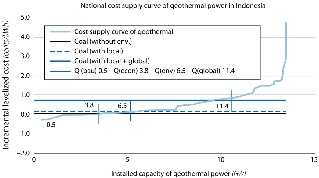
Figure 4.17 Geothermal Power in Indonesia Is Economically Competitive with Coal-Based Power (cents/kWh)
