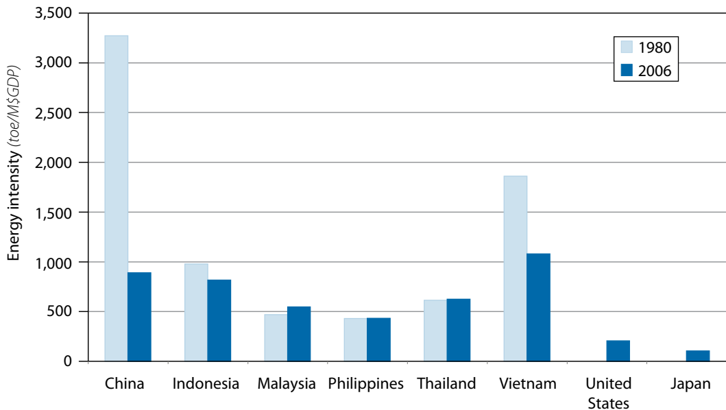
Figure 1.5 China and Vietnam Significantly Reduced Energy Intensity Whereas Other East Asian Countries Increased It, 1980–2006, but Region Lags behind Developed Countries ( toe/M$GDP )
