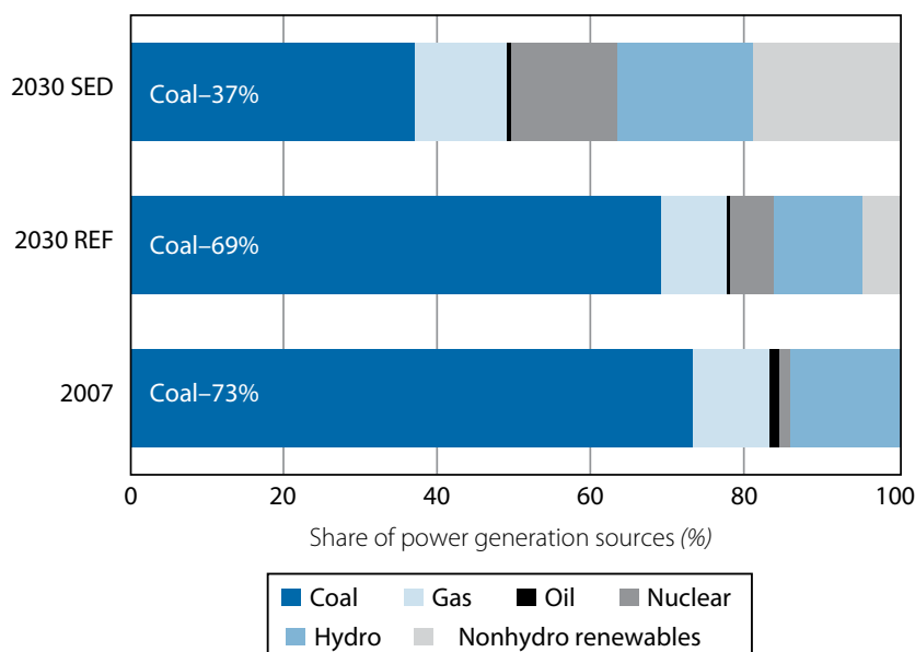
Figure 2. Power Generation Will Need to Shift Dramatically from Coal to Renewable Energy and Nuclear Power, 2007–30 (%)
