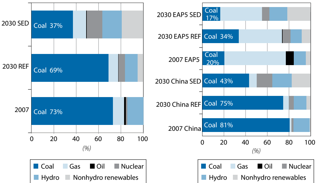
Figure 4.16 Under the SED Scenario, Power Generation Shifts Dramatically from Coal to Renewable Energy and Nuclear Power (EAP Region; EAP5 and China) (%)
